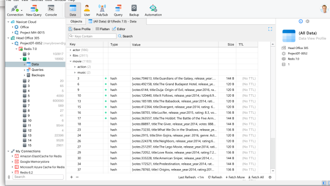
Linux Version
